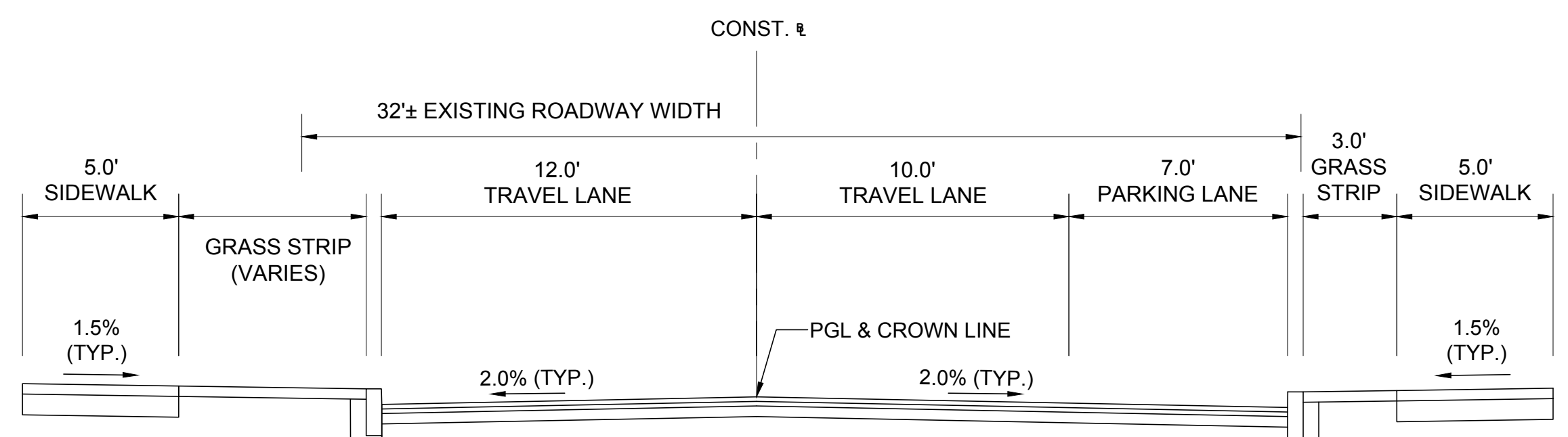
TYPICAL SECTION - BOYLSTON STREET (WEST OF SCHOOL STREET) SCALE: N.T.S.
