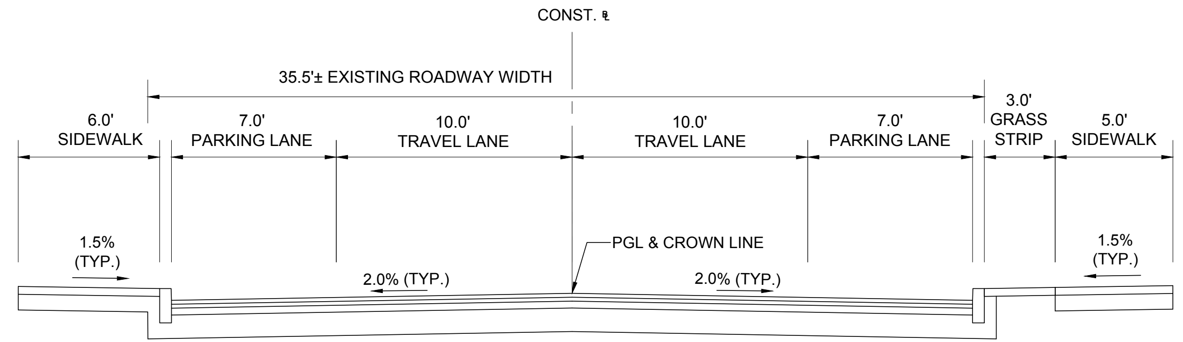
TYPICAL SECTION - BOYLSTON STREET (WEST OF SCHOOL STREET) SCALE: N.T.S.
